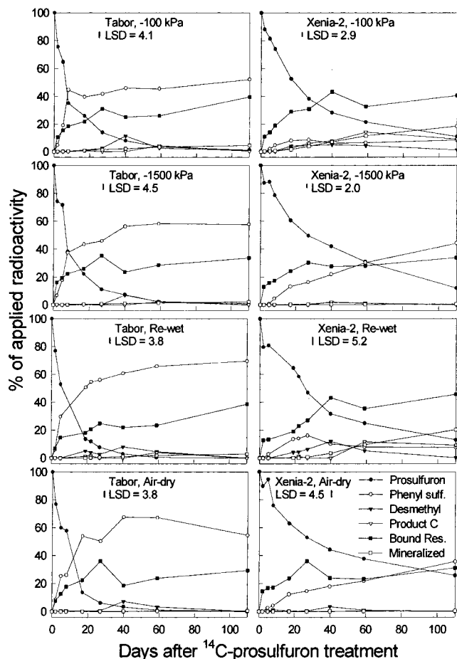
Figure 5. Distribution of ^{14}\text{C} in extractable, bound residue, and mineralized ( ^{14}\text{CO}_2 ) phases in soil water content study. Extractable phase represented by HPLC detection of ^{14}\text{C} -labeled compounds: prosulfuron, phenyl sulfonamide, desmethyl prosulfuron, and product C.
