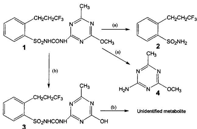
Figure 1. Structures of prosulfuron (1), phenyl sulfonamide (2), desmethyl prosulfuron (3), and amino triazine (4). Only 1–3 were traceable in this study. Proposed degradation pathways of prosulfuron in soil: (a) chemical hydrolysis and (b) microbial degradation. See text for discussion of degradation product of 3 detected in soil incubations.
