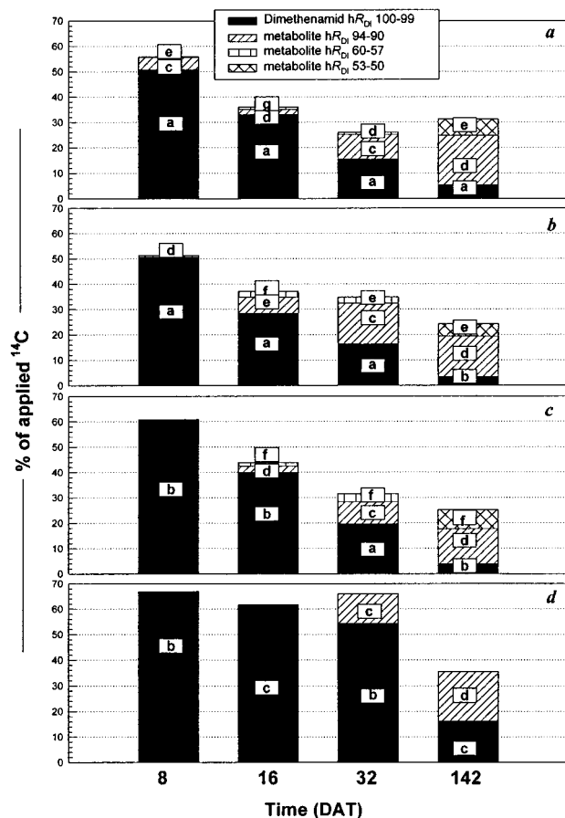
Figure 4. Distribution of [ ^{14}\text{C} ]dimethenamid, nonpolar, and polar ^{14}\text{C} -metabolites in the glucose-amended, unamended, \text{NO}_3^- + \text{SO}_4^{2-} -amended, and autoclaved treatments at 8, 16, 32, and 142 DAT. The boxed letters are for comparing treatments on the same day and denote differences at the 5% probability level ( n = 3 ). (a) Glucose-pretreated microcosms, (b) unamended microcosms, (c) nitrate + sulfate-amended microcosms, and (d) autoclaved microcosms.
