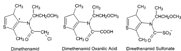
Figure 1. Chemical structures of dimethenamid, dimethenamid oxalamic acid, and dimethenamid sulfonate. The asterisk denotes the position of the radiolabel in dimethenamid.
